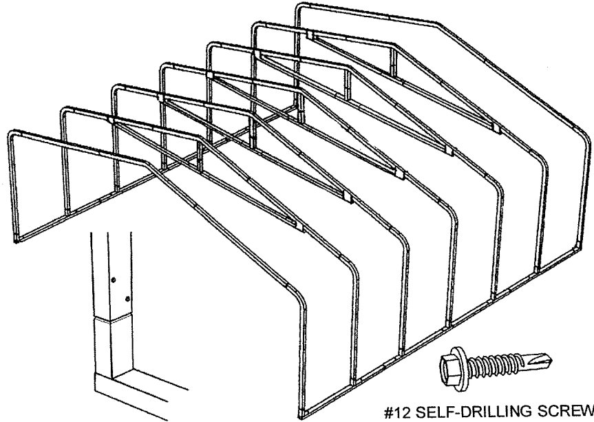
SQUARING UP YOUR FRAME
